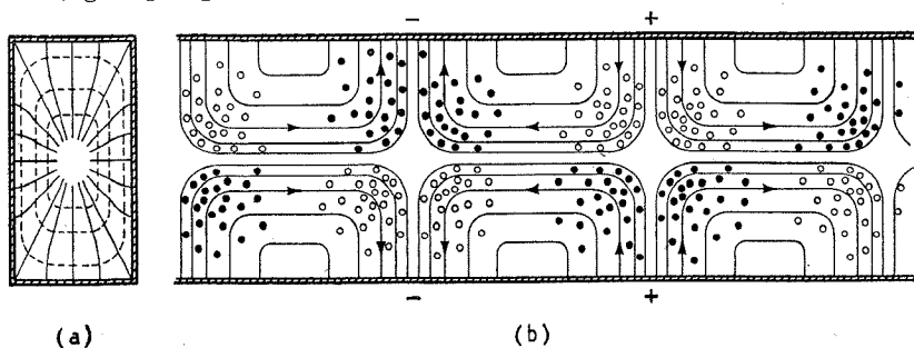
Fig. 12. End and side views of a guide with E_{11} waves. The magnetic loops are transverse instead of longitudinal as in the H waves, while the electric field is partly longitudinal. In the side view (b) the magnetic loops are shown in section, black dots indicating direction up from the paper and white circles direction into the paper.
