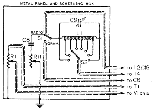
Fig. 2. Screening arrangements required when rejector circuit is mounted outside the cabinet as a remote control unit. C9 must be insulated from panel.
