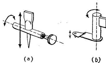
Fig. 3. (a) Conventional pick-up movement. (b) Redesigned movement with reduced inertia for vertical motion.
