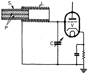
Permeability tuner.
