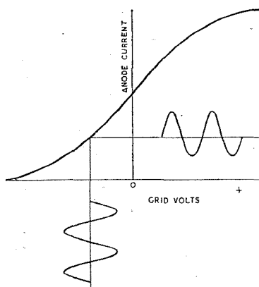
Fig. 1. Grid-volts/anode-current characteristics with Class "A" operation.
