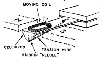
Fig. 7. Simple moving coil pick-up using the hairpin needle principle.
