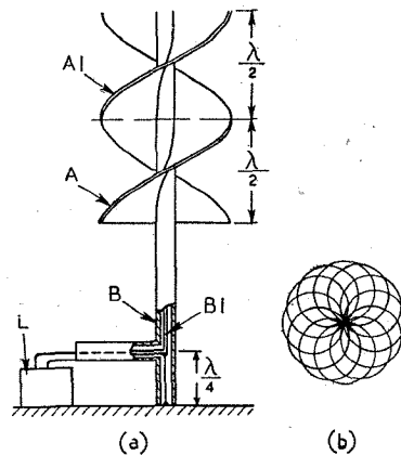
(a) (b) Omnidirectional aerial.
