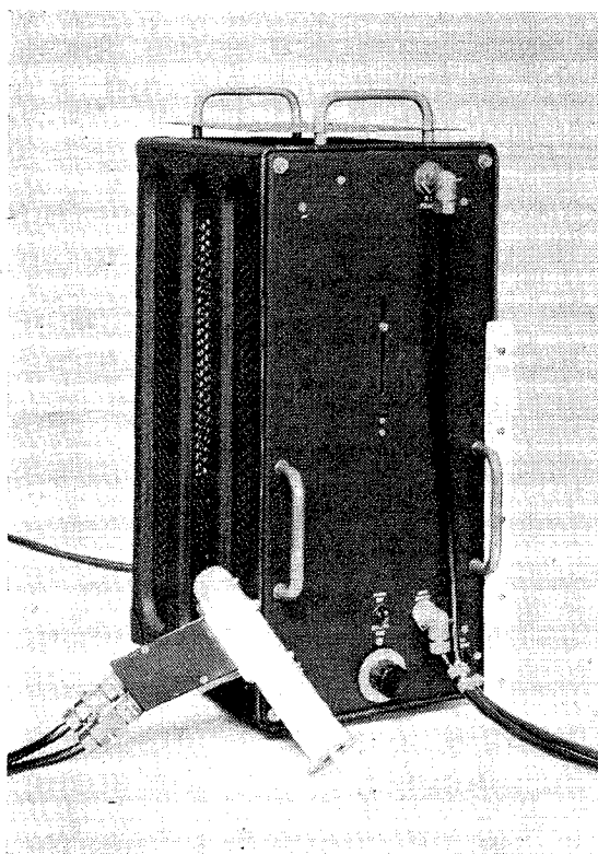
Portable RF "spot gluing" equipment developed by Pye Telecommunications, Ltd., for Aero Research, Ltd.
